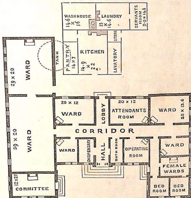
GROUND PLAN.
