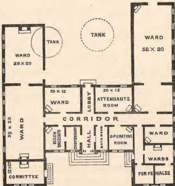
GROUND PLAN.
