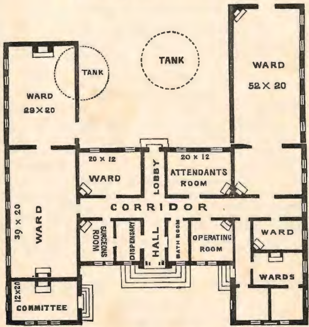
GROUND PLAN.
